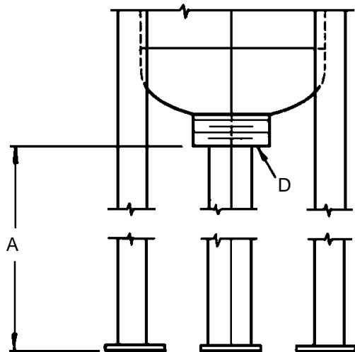
Flanged Connections
