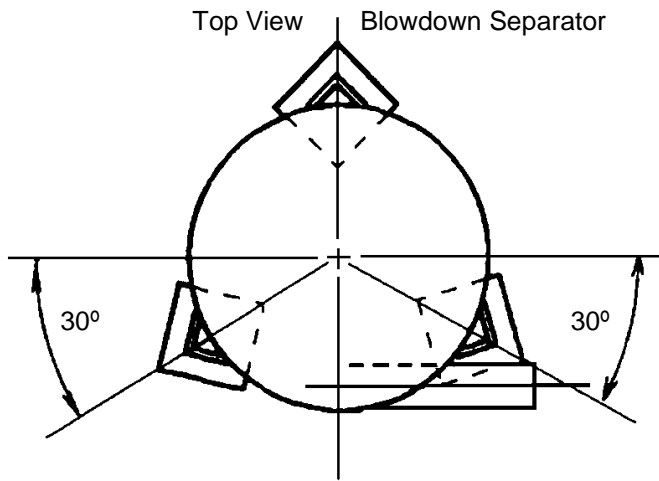
Screwed or Beveled Connections
